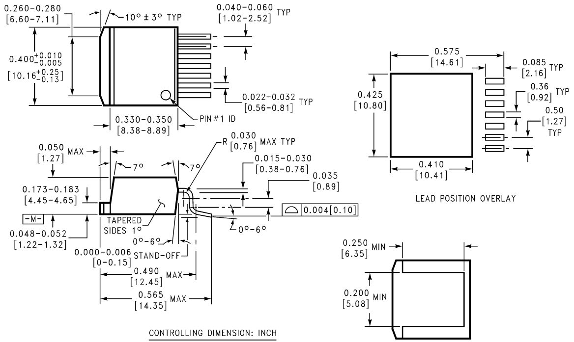
TO-263 Surface Mount Power Package Order Number LM2676S-3.3, LM2676S-5.0, LM2676S-12 or LM2676S-ADJ NS Package Number TS7B
